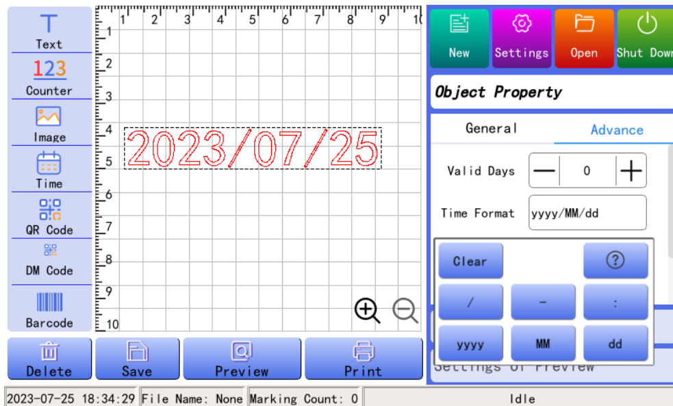
Figure 3.2.4.1 Time Edit
