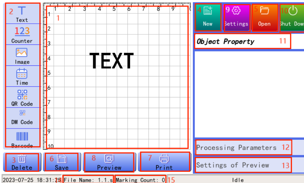
Figure 3.1.1 Main interface3.1.1
